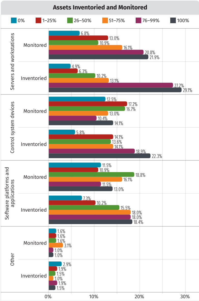
Figure 22. Percentage of Monitored/Inventoried Assets
