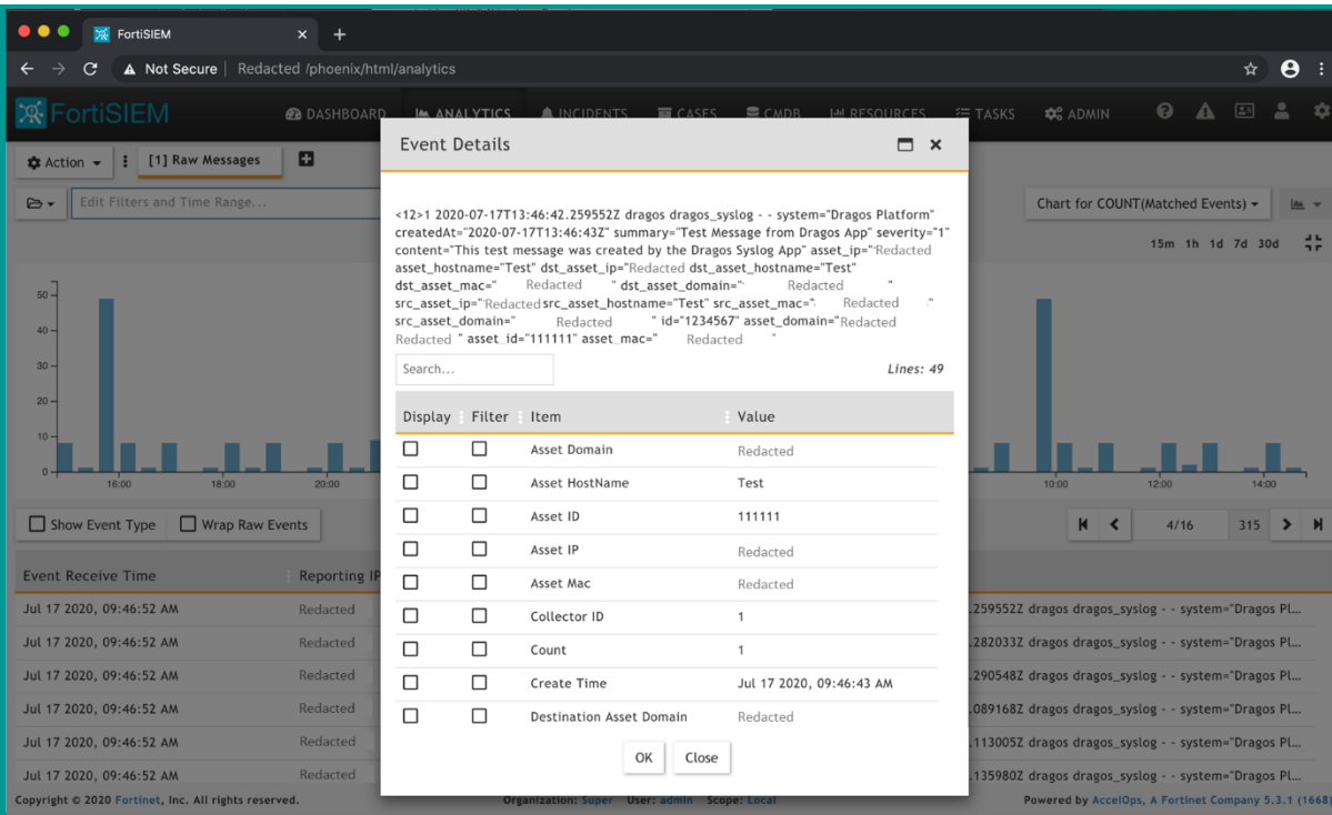
Figure 2. FortiSIEM with Dragos Platform data displayed.
