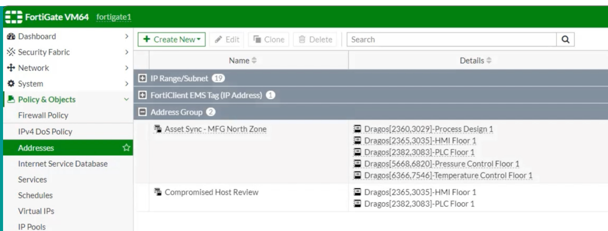
Figure 1. FortiGate address groups populated by the Dragos Platform.
