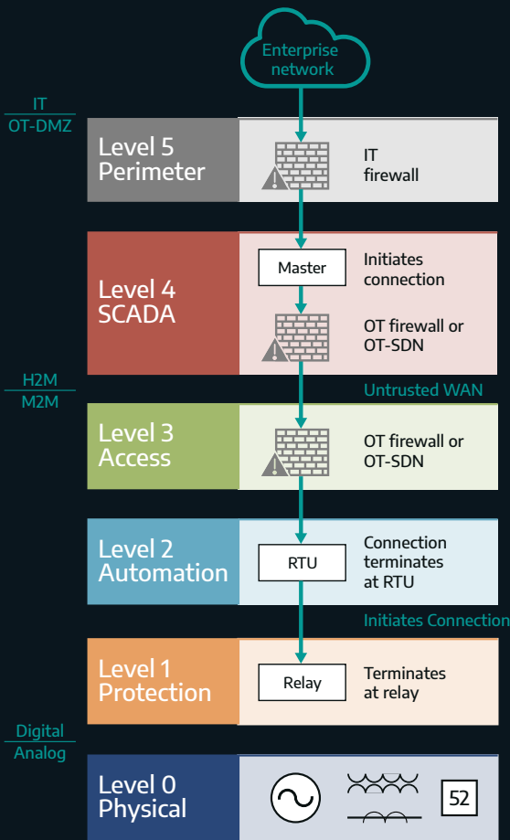
FIG. 2 LAYERED CYBERSECURITY FOR A UTILITY OT NETWORK
