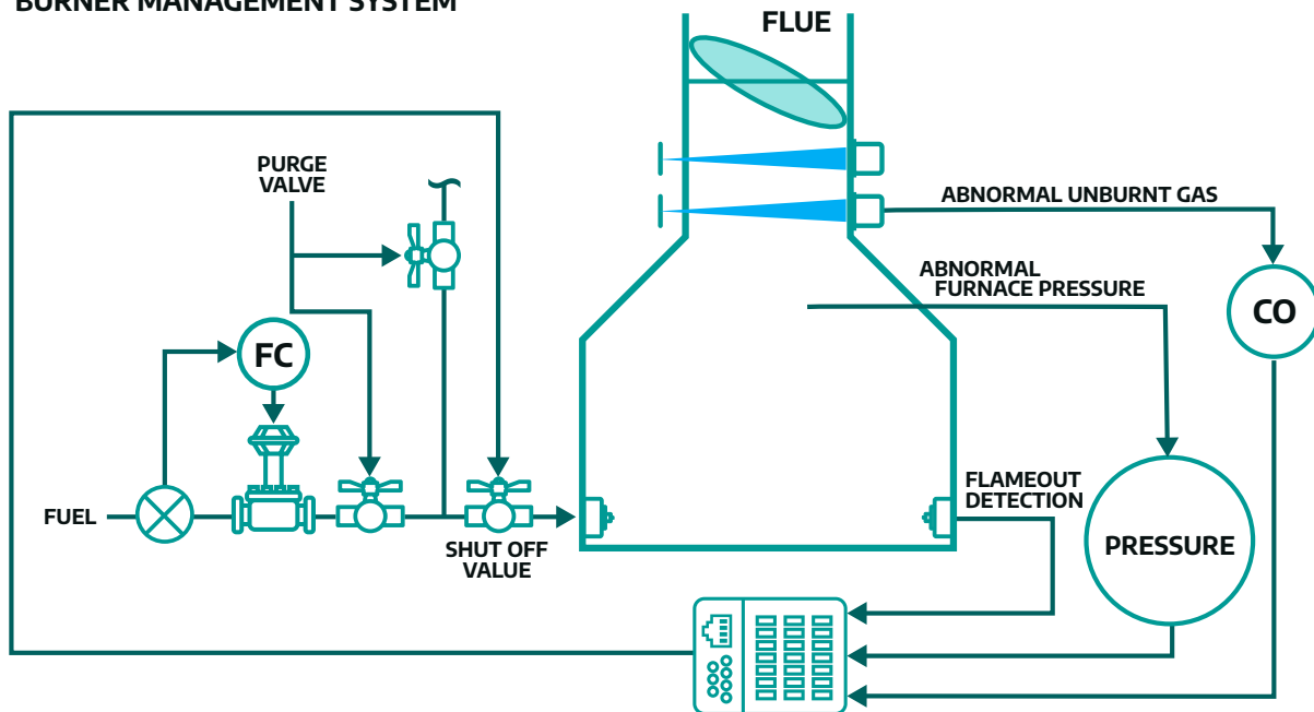
BURNER MANAGEMENT SYSTEM
