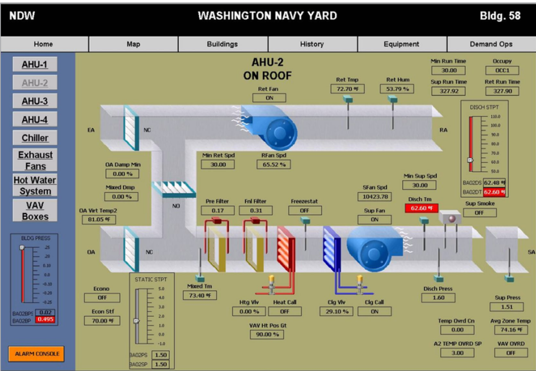
Figure 8. Building HVAC Human Machine Interfaces
