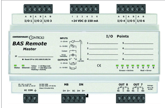
Figure 28. 2A-CC: Very basic Level 2A controller capable of monitoring six analog inputs and reporting their values to the network and setting two outputs. The network is BACnet over IP over 10/100Mbps.
